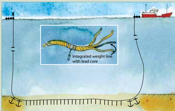
Figure 1. Autoline gear configuration.
